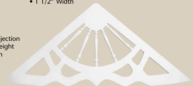
GB 6733 • 1" Projection • 40 1/2" Height • 81" Width • 12/12 Pitch
